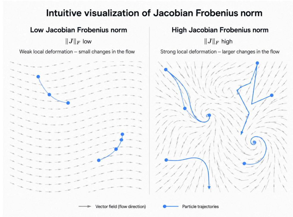
Figure 1: Conceptual visualization of the Frobenius norm \|J\|_F as a measure of total local flow deformation. Left: low \|J\|_F — nearby particle trajectories (blue) through the local vector field (grey arrows) remain smooth and close together. Right: high \|J\|_F — trajectories through the same class of local vector field are strongly bent, twisted, and redirected, reflecting large aggregate deformation across all directions. Schematic illustration for methodological intuition only; not derived from ds004511 data.
