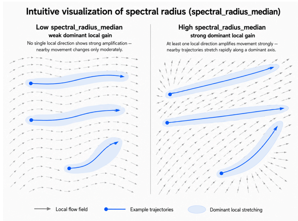
Figure 2: Conceptual visualization of the spectral radius \rho(J) = \max_i |\lambda_i(J)| as a measure of dominant local gain. Left: low \rho(J) — no single local direction shows strong amplification, so nearby trajectories change only moderately regardless of starting orientation. Right: high \rho(J) — at least one local direction amplifies movement strongly, so nearby trajectories stretch rapidly along a dominant axis (shaded bands) while other directions may remain comparatively unamplified. Schematic illustration for methodological intuition only; not derived from ds004511 data.
